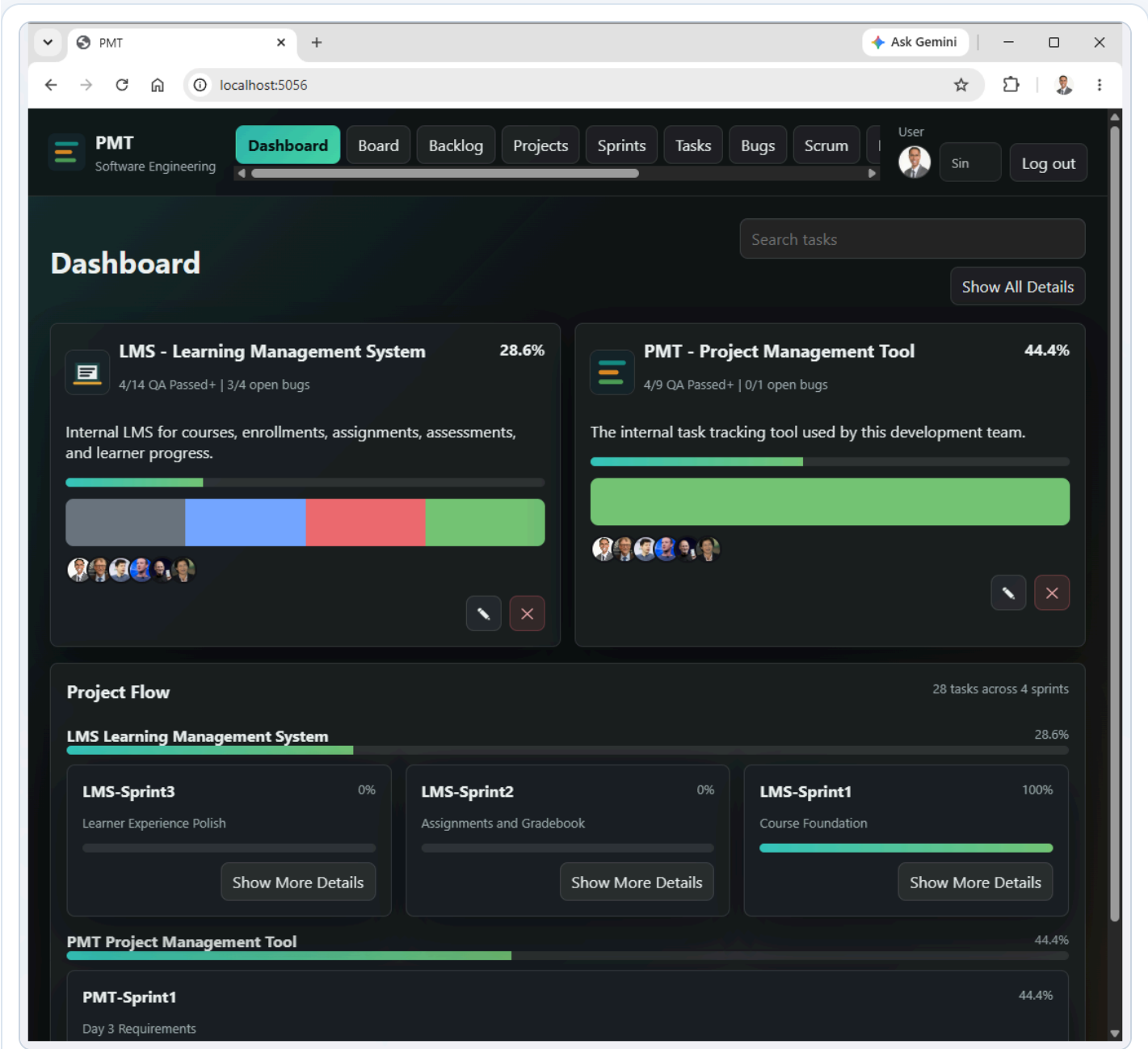
Dashboard showing project health, sprint flow, progress bars, team avatars, and detail controls.
